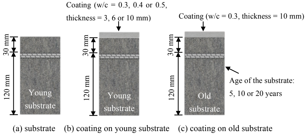
Fig. 10 Schematic illustration of (a) substrate, (b) coating on young substrate, and (c) coating on old substrate systems. The coatings with different w/c ratios and thicknesses are applied on young/old substrates.
