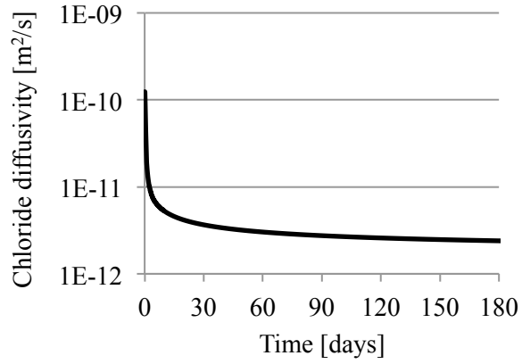
(a) Coating ( w/c = 0.3 )
