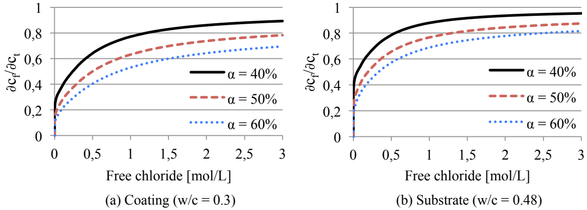
Fig. 9 Ratio of free chloride to total chloride, \partial C_f / \partial C_t , accounting for chloride binding capacity of the (a) coating (w/c = 0.3) and (b) substrate (w/c = 0.48).
