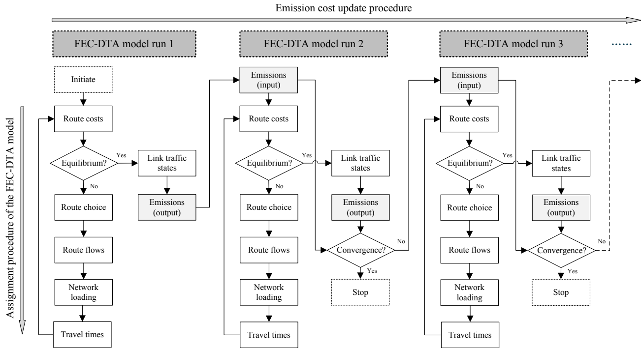
FIGURE 1 Conceptual flow chart of the bi-level optimization method used to solve the dynamic traffic assignment problem with multi-criteria routing
