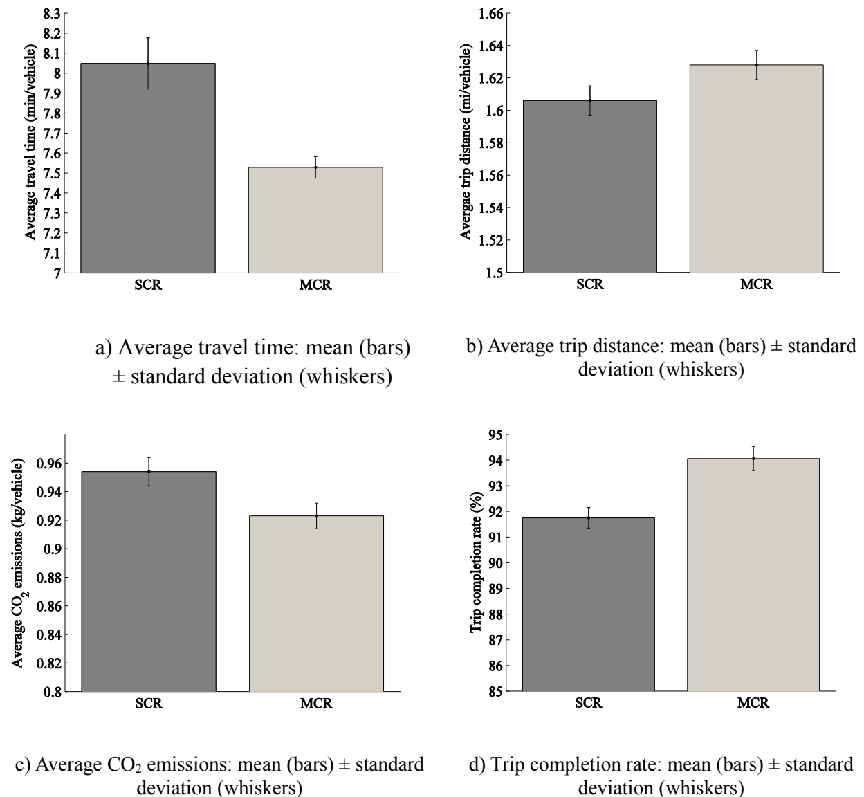
FIGURE 4 Network performance in the SCR and MCR scenarios.
