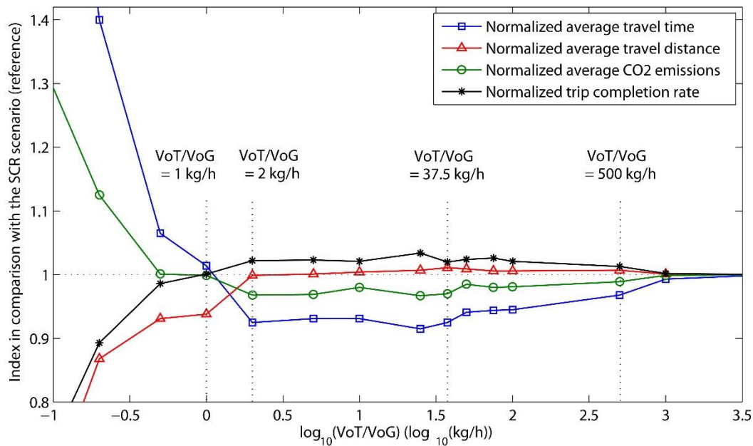
FIGURE 5 Network performance with different VoT/VoG ratios. Note that the scale of the horizontal axis is logarithmic. The reference case corresponds to the single-criteria routing scenario (in which emission costs are not included in the route cost function)
