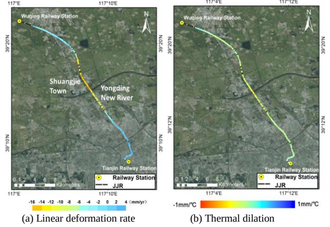
Fig. 4. Linear deformation rate and thermal dilation maps of JJR (2008-2009). Background image: Google Map.
