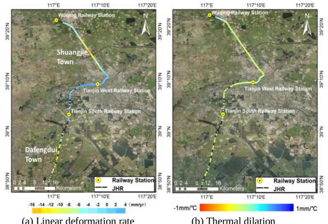
Fig. 5. Linear deformation rate and thermal dilation maps of JHR (2008-2009). Background image: Google Map.
