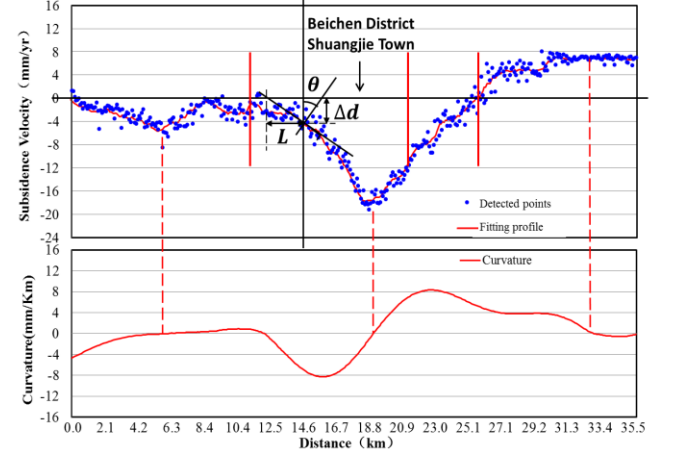
(b) Subsidence rate profile and curvature of JJR
