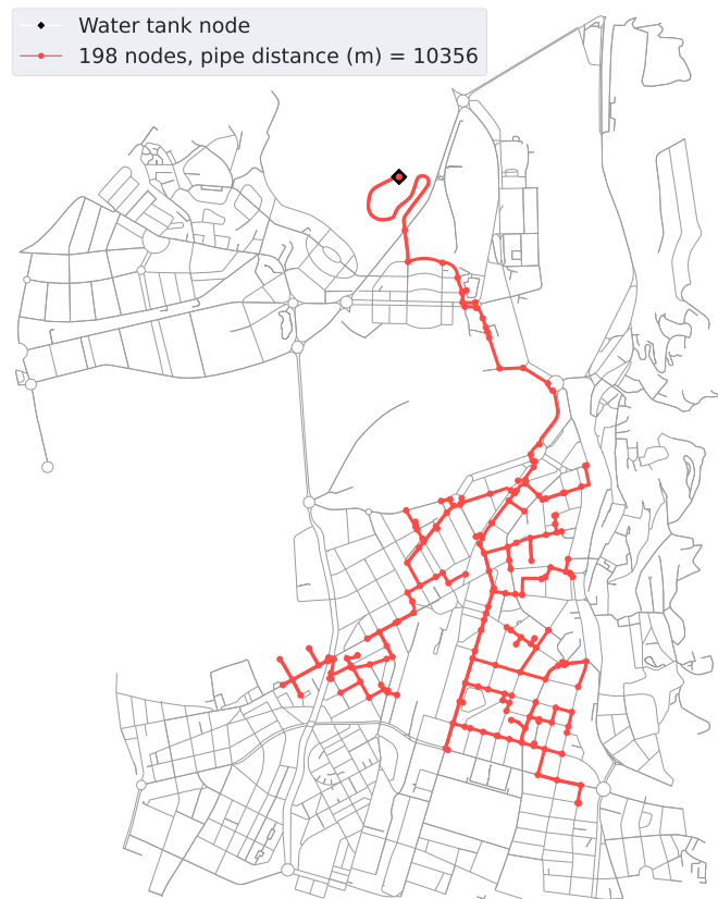
Fig. 3. Visualization of the ‘non-resilient’ current reclaimed water network in Girona (highlighted in red) overlaying the Girona street graph (in grey).
