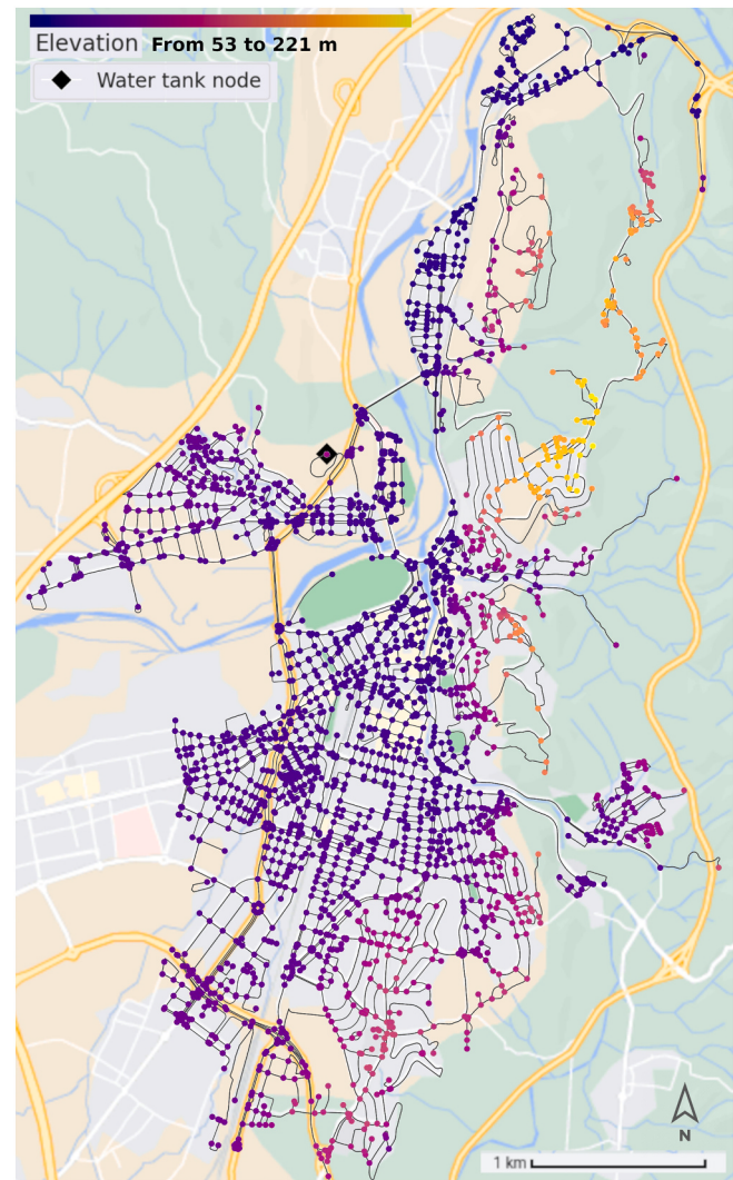
Fig. 1. Visualization of the Girona case study area, highlighting nodes color-coded by elevation, and indicating the placement of the initial water tank.
