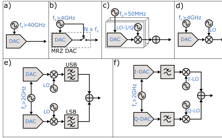
Fig. 3. Possible transmitter architectures: (a) Very high speed DAC, (b) MRZ DAC, (c) low speed DAC with mixer, (d) high speed DAC with mixer (e) SSB modulation with band pass filters for the sidebands, (f) High speed DAC with reconstruction filter and I/Q mixer.
