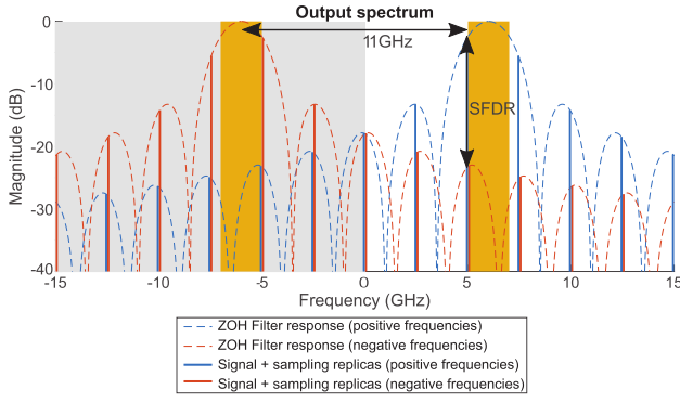
Fig. 6. Output spectrum assuming an output tone around 5 GHz, a carrier frequency of 6 GHz, a sample rate of 2.5 GHz, and no reconstruction filter.
