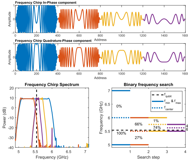
Fig. 14. Binary search for the qubit resonance frequency using multiple frequency chirps. Top: the in-phase and quadrature-phase envelopes used in the different cycles of the search. Bottom-left: the resulting spectra of the frequency chirps. Bottom-right: the start/stop/center frequency in every cycle of the search protocol, along with the simulated probability of finding the qubit in the excited state after performing the chirp, which determines the next chirp frequency band.
