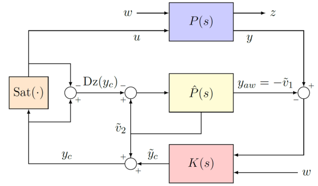
Fig. 19 MRAW architecture
