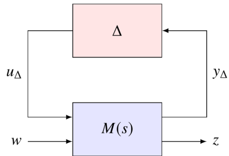
Fig. 7 LFR of a system with parametric uncertainties
