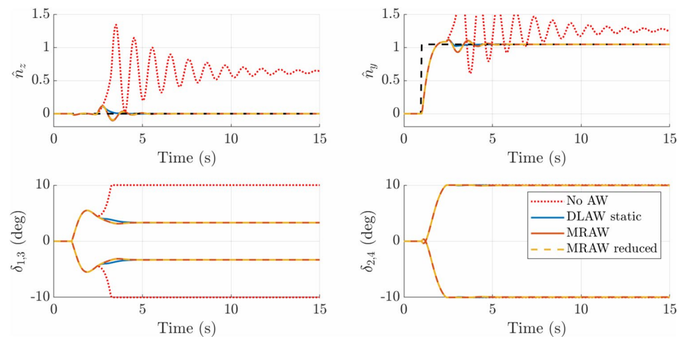
Fig. 20 Step responses for different anti-windup schemes
