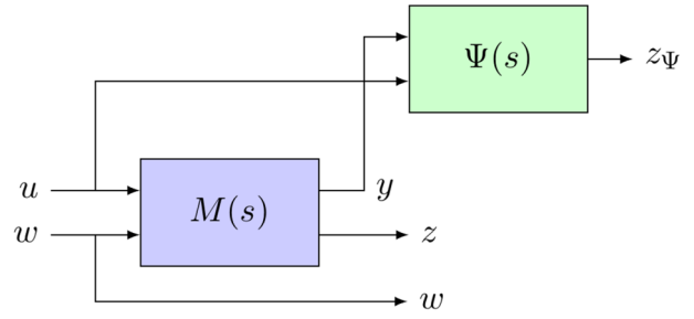
Fig. 21 IQC performance analysis
