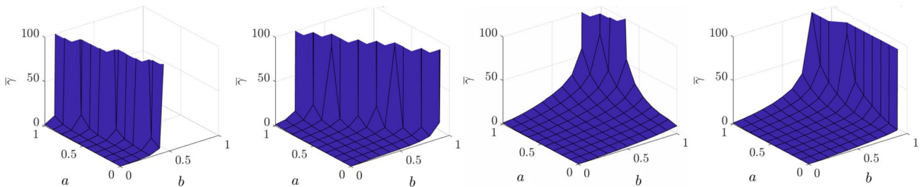
Fig. 22 Bounds on the \mathcal{L}_2 -gain in the presence of aerodynamic uncertainties |\delta_a| \leq a and nonlinearity \Phi \in \sec[0, b]^2 \cap \text{slope}[0, b]^2 ; from left to right: no anti-windup, static DLAW, MRAW, reduced MRAW
