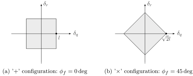
Fig. 18 Set of virtual control signals leading to no saturation
