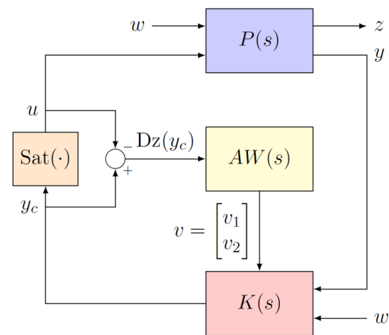
Fig. 16 Principle of anti-windup compensation
