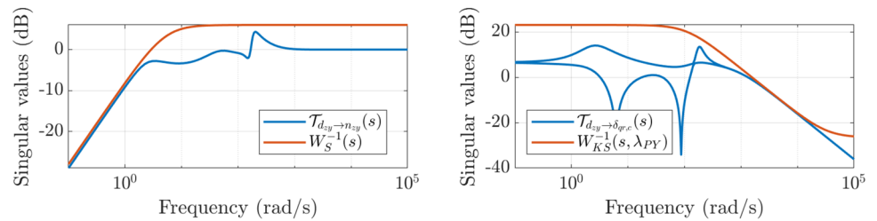
Fig. 12 Closed-loop transfer functions for disturbance rejection (left) and control attenuation (right)
