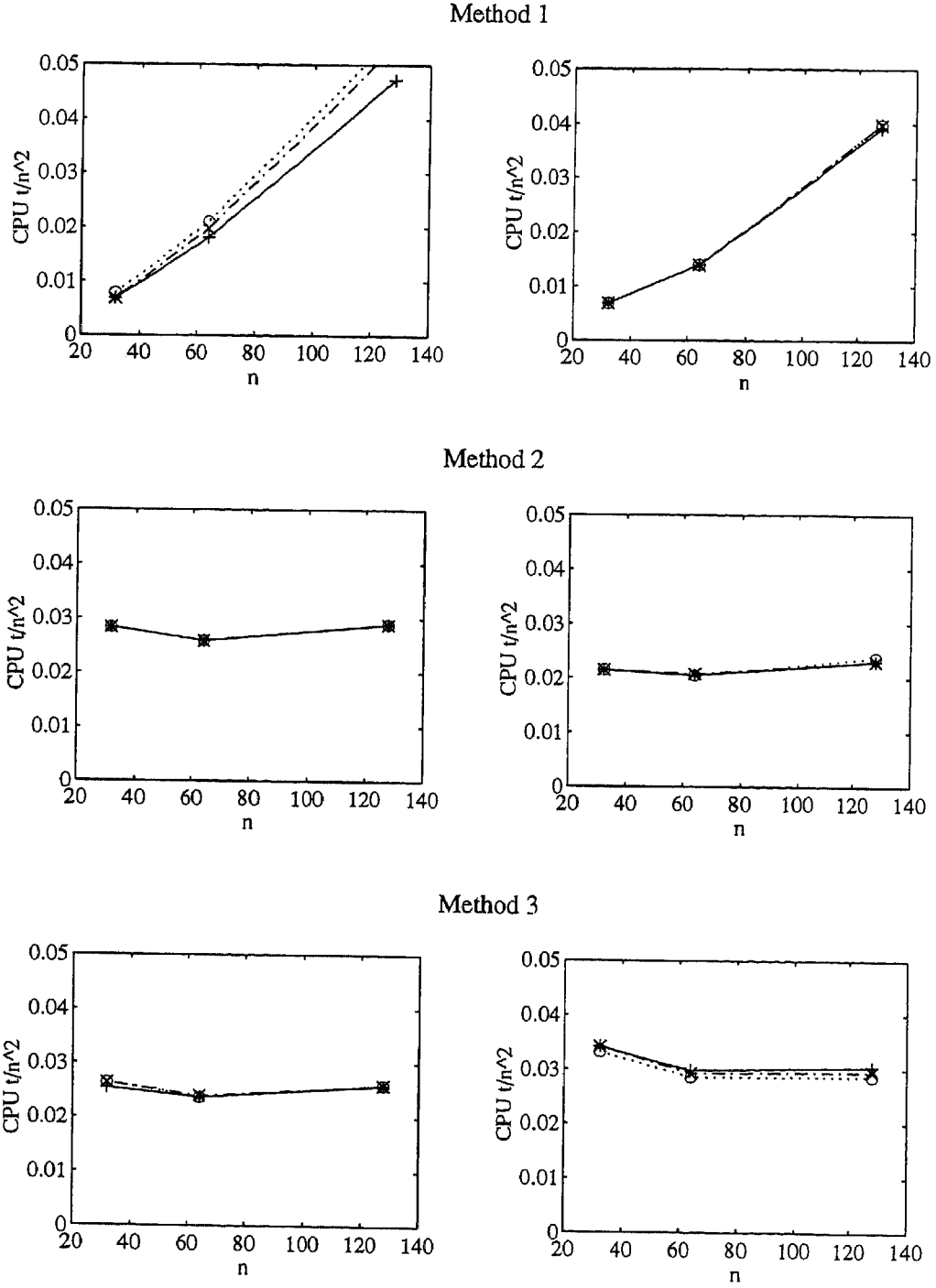
Figure 3.5: Problem 3 at Re = 1 on the HP: CPU time per grid point on different grids for the solution of the momentum equations (left) and for the solution of the pressure equation (right). Solid lines and plus marks: \Delta t = 0.0625 ; dashdot lines and x-marks: \Delta t = 0.125 ; dotted lines and circles: \Delta t = 0.25
