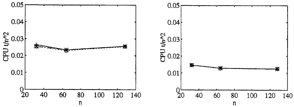
Figure 3.7: Problem 4 at Re = 1 on the HP: CPU time per grid point on different grids for the solution of the momentum equations (left) and for the solution of the pressure equation (right). Solid lines and plus marks: \Delta t = 0.0625 ; dashdot lines and x-marks: \Delta t = 0.125 ; dotted lines and circles: \Delta t = 0.25
