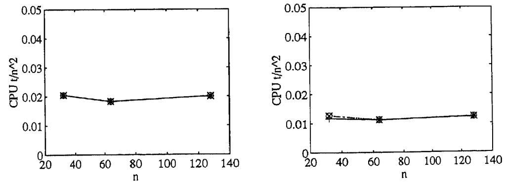
Figure 3.4: Problem 2 at Re = 1000 on the HP: CPU time per grid point on different grids for the solution of the momentum equations (left) and for the solution of the pressure equation (right). Solid lines and plus marks: \Delta t = 0.0625 ; dashdot lines and x-marks: \Delta t = 0.125 ; dotted lines and circles: \Delta t = 0.25
