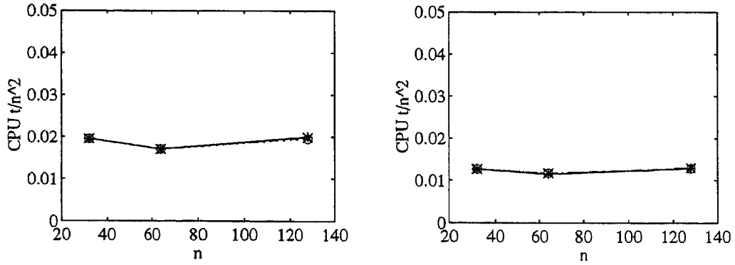
Figure 3.3: Problem 2 at Re = 1 on the HP: CPU time per grid point on different grids for the solution of the momentum equations (left) and for the solution of the pressure equation (right). Solid lines and plus marks: \Delta t = 0.0625 ; dashdot lines and x-marks: \Delta t = 0.125 ; dotted lines and circles: \Delta t = 0.25
