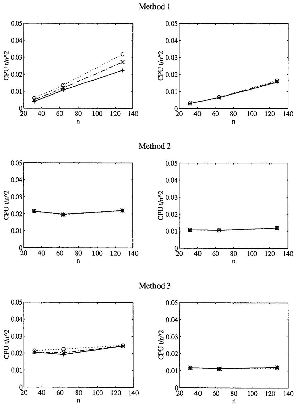
Figure 3.1: Problem 1 at Re = 1 on the HP: CPU time per grid point on different grids for the solution of the momentum equations (left) and for the solution of the pressure equation (right). Solid lines and plus marks: \Delta t = 0.0625 ; dashdot lines and x-marks: \Delta t = 0.125 ; dotted lines and circles: \Delta t = 0.25
