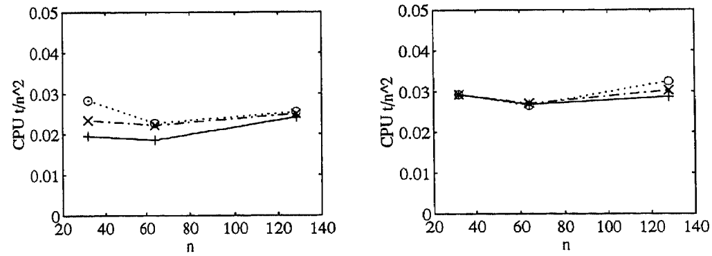
Figure 3.6: Problem 3 at Re = 1000 on the HP: CPU time per grid point on different grids for the solution of the momentum equations (left) and for the solution of the pressure equation (right). Solid lines and plus marks: \Delta t = 0.0625 ; dashdot lines and x-marks: \Delta t = 0.125 ; dotted lines and circles: \Delta t = 0.25
