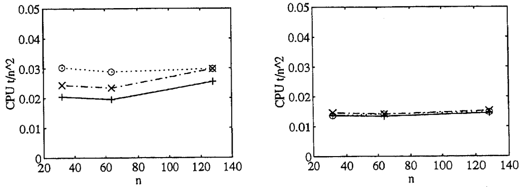
Figure 3.8: Problem 4 at Re = 1000 on the HP: CPU time per grid point on different grids for the solution of the momentum equations (left) and for the solution of the pressure equation (right). Solid lines and plus marks: \Delta t = 0.0625 ; dashdot lines and x-marks: \Delta t = 0.125 ; dotted lines and circles: \Delta t = 0.25
