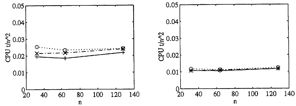
Figure 3.2: Problem 1 at Re = 1000 on the HP: CPU time per grid point on different grids for the solution of the momentum equations (left) and for the solution of the pressure equation (right). Solid lines and plus marks: \Delta t = 0.0625 ; dashdot lines and x-marks: \Delta t = 0.125 ; dotted lines and circles: \Delta t = 0.25
