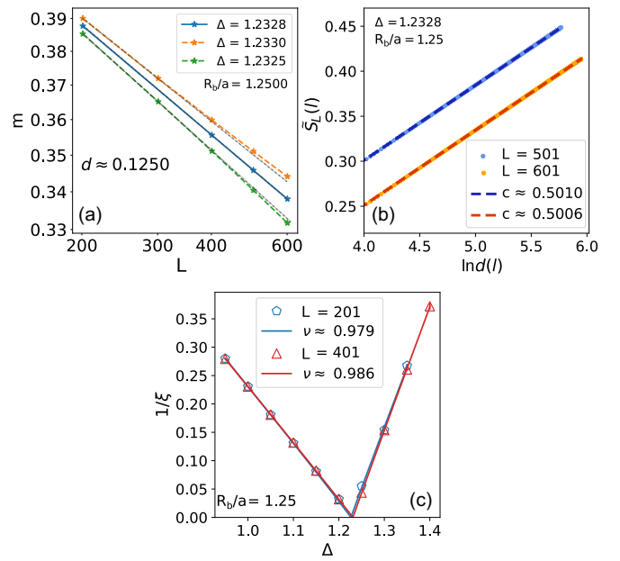
FIG. 6. Numerical extraction of the critical exponents for the transition out of the \mathbb{Z}_2 phase. (a) Finite-size scaling of the order parameter m = \hat{a}_i in the middle of a finite-size chain in a log-log scale. We identify the location of the critical point by the separatrix. To better highlight the curvature of the scaling curves, straight dashed lines are included as visual guides. The extracted scaling dimension d is in excellent agreement with the CFT prediction for Ising transition d = 1/8 . (b) Scaling of the entanglement entropy \tilde{S}_L with the conformal distance d(l) after removing Friedel oscillations. Results for L = 601 where shifted by -0.05 for clarity. The slope agrees with the Ising central charge c = 1/2 . (c) Scaling of the inverse of the correlation length 1/\xi in the vicinity of the transition, extracted from the density-density correlations of the operator \hat{a} . The extracted critical exponent \nu agrees with the theory prediction \nu = 1 .
