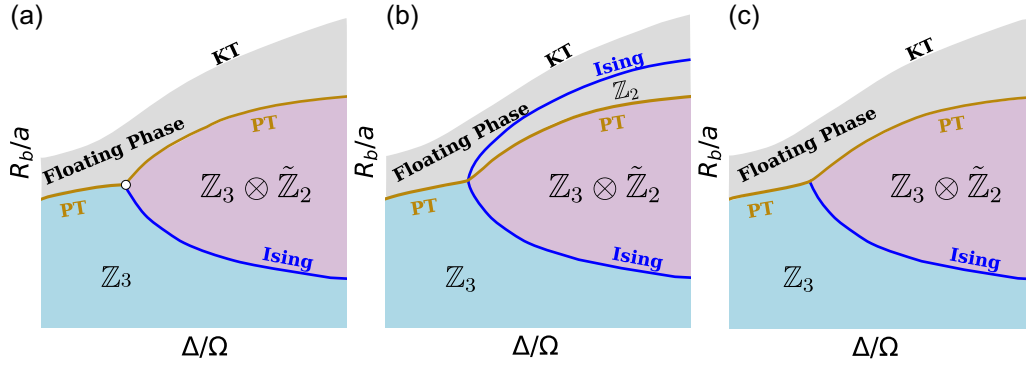
FIG. 15. Sketch of the three possible scenarios for the multicritical point where the floating Z_3 and Z_3 \otimes \tilde{Z}_2 phases meet. (a) The Ising and Pokrovsky-Talapov lines meet at a multicritical point. (b) The Ising critical line extends inside the floating phase as a higher-symmetry line separating two regions of the floating phase with spontaneously broken \tilde{Z}_2 symmetry in one of them. (c) The Ising transition takes place higher in the energy spectrum after crossing the Pokrovsky-Talapov transition.
