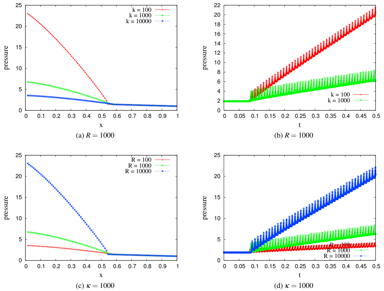
Figure 5 (Left) pressure versus spatial coordinate at t = 0.1 , (Right) pressure versus time at x = 0.5 , of the foam model with resolution N = 100 and M = 1 , S_w^* = 0.2 , p_L = 11 , p_R = 1 .
