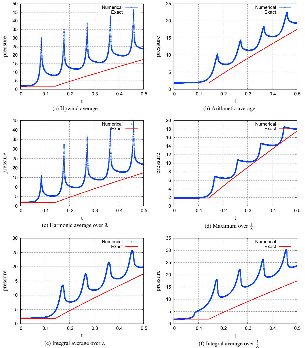
Figure 15: Pressure vs time at x = 0.15 for N = 10 , M = 1 , S_w^* = 0.2 , with u_L = 10 described on the left boundary and p_R = 1 prescribed on the right boundary.
