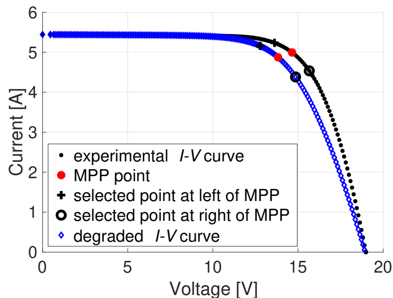
Figure 4. Healthy and degraded I - V curves with the selected points passed to the ANN.
