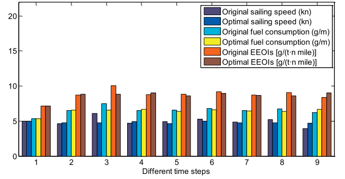
Fig. 13. The navigation optimization results of the 5# ship.
