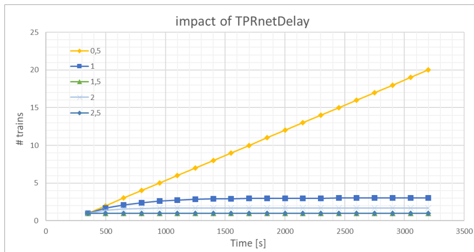
Figure 15. No. of trains versus simulated time for different values of TPRnetDelay
