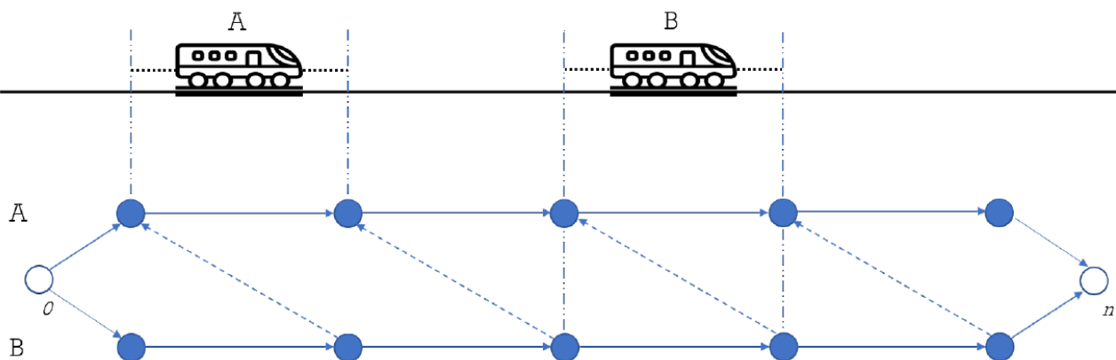
Figure 5. Alternative graph for two trains on a single track under moving-block signalling with virtual nodes in blue. Adapted from (Janssens, 2022).
