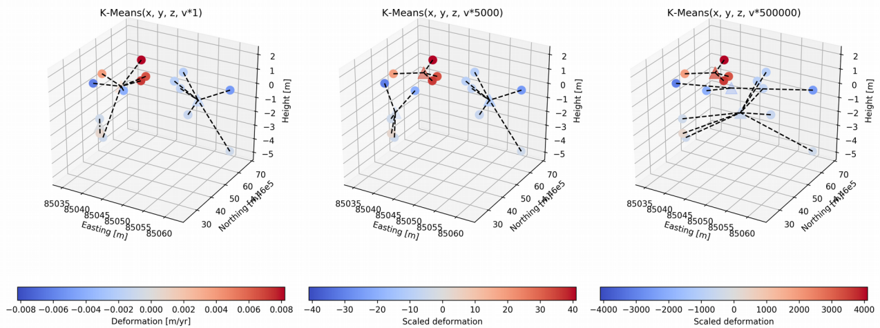
Figure 24: Clusters of data, with increased scaling of the velocity component. Input points are shown as circles, centroids as pyramids.
