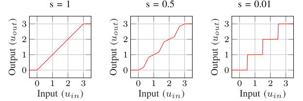
Fig. 4. A 2-bit Soft-DAC activation unit for different softening factor ( s ).
