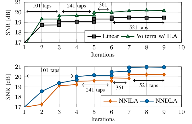
Fig. 6. Training of different DPDs at 460 mV DACs' voltage by increasing the memory length of the 4 \times 4 real-valued MIMO equalizer in the receiver DSP.
