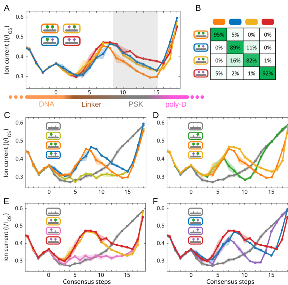
Figure 4. Charged residues on the peptide dominate nanopore signals. (A) Consensus traces for the double-modification variants. The shaded area highlights the steps with the largest current difference where the pentapeptide translocates the nanopore constriction. (B) Confusion matrix of the double-modification variants. The most difficult calling is between the sY-pY and pY-sY isomers. (C–F) Signal consensus of variants carrying sulfation on 1st tyrosine (A), sulfation on 2nd tyrosine (B), phosphorylation on 1st tyrosine (C), and phosphorylation on 2nd tyrosine (D). The unmodified peptide (gray) is used as a reference trace in all plots. Higher negative charge on the peptide leads to a higher current in general.
