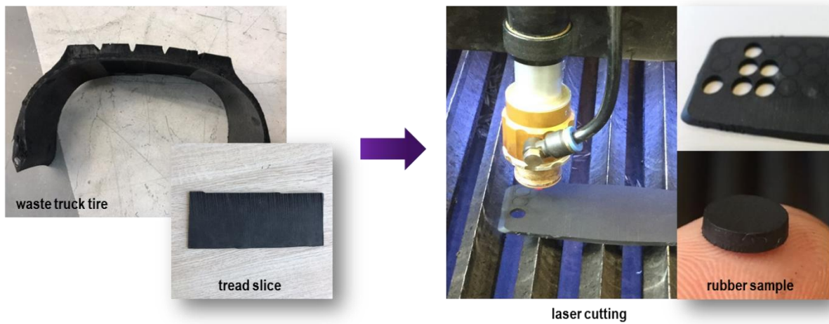
Figure 1. Cylindrical rubber sample (2 mm-thickness and 8 mm-diameter) preparation process.
