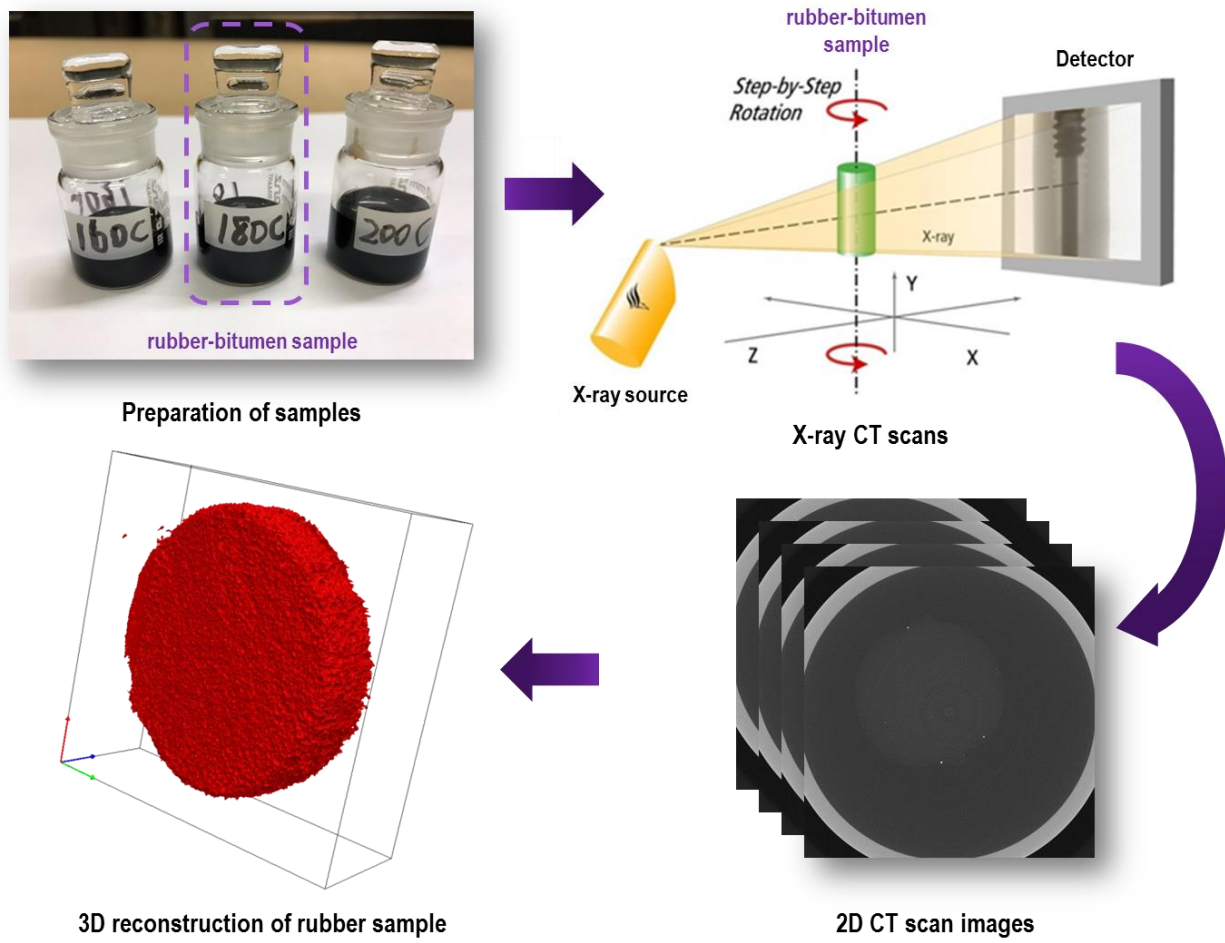
Figure 2. X-ray CT scan test for monitoring the rubber swelling process.
