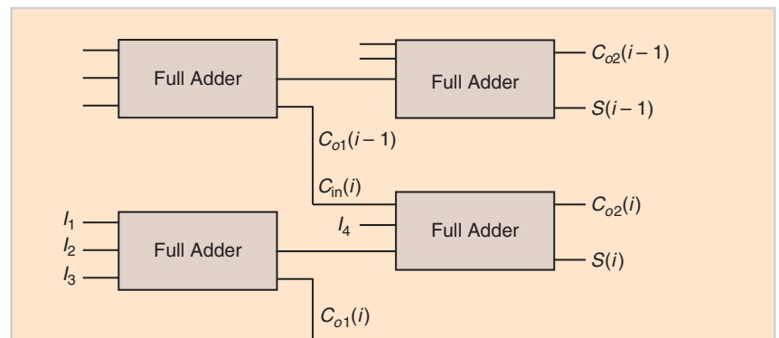
FIGURE 4 A 4:2 compressor.
