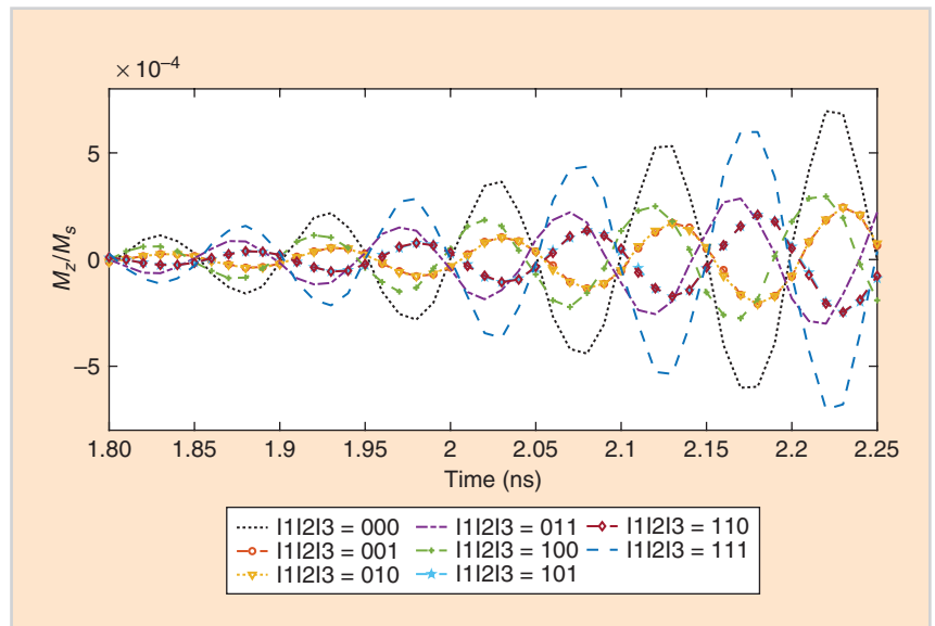
FIGURE 8 The normalized 4:2 compressor output C_{01} .
