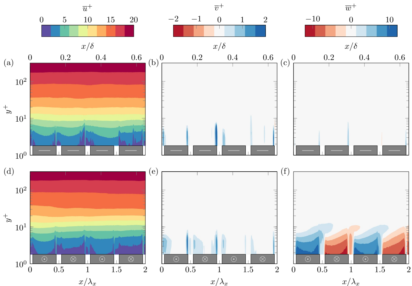
Fig. 2 Scalar fields of the mean streamwise velocity ( a,d ), the mean wall-normal velocity ( b,e ), and the mean spanwise velocity ( c,f ), for the non-actuated case (top row) and actuated case (bottom row) at A^+ = 12.7 . The grey-shaded regions indicate the belt locations and
