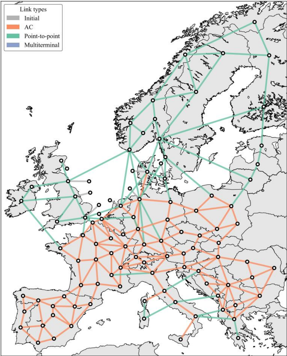
Figure 5.3: 2030 initial system
