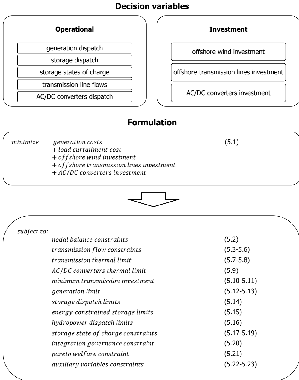
Figure 5.2: Single period expansion model formulation
