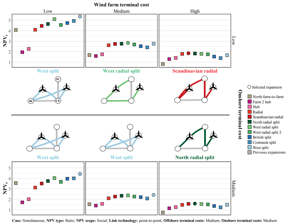
Figure 4.9: Influence of comparative terminal investment costs
