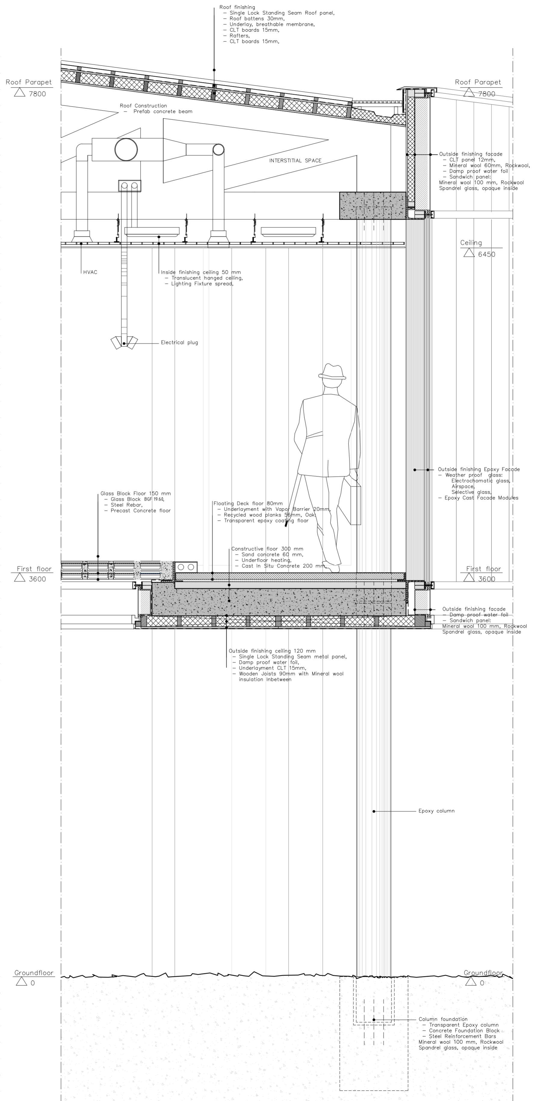
Cross Section
