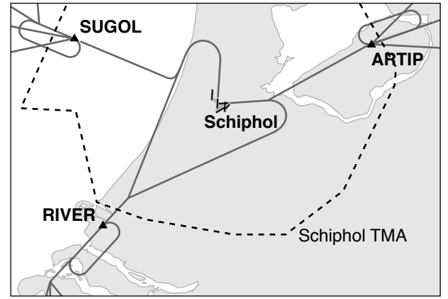
Fig. 1. Approach routes in simulation.
