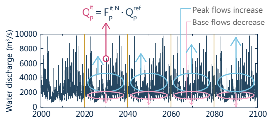
Figure B.12: Procedure to transform a reference cycled hydrograph into a scenario cycled hydrograph using the statistics of the Sperna-Weiland et al. (2015) water discharge scenarios.
