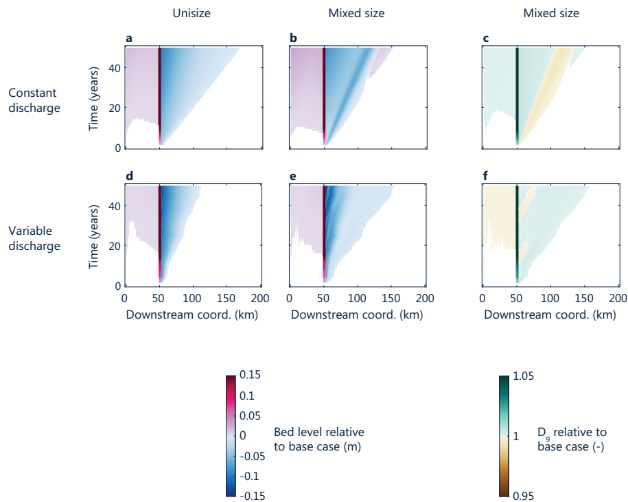
Figure 4.5: Space-time plots of simulated bed level change and bed surface grain size change due to an erosion control measure, relative to a base case without the measure: (a) constant discharge - unisize sediment; (b,c) constant discharge - mixed-size sediment; (d) variable discharge - unisize sediment; (e,f) variable discharge - mixed-size sediment.
