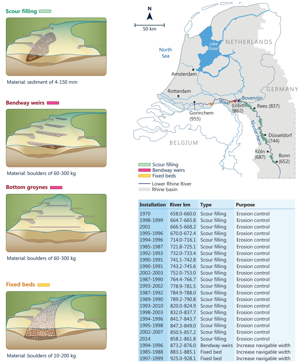
Figure 4.1: Erosion control measures in the lower Rhine River, with details on their installation period, location, type, and main purpose.
