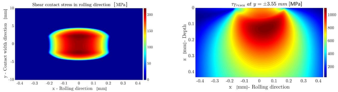
Figure 7: Exemplary presentation of the calculated: (a) Shear contact stress in rolling direction and (b) Tresca stress at the position of maximum p \cdot v_{\text{sliding}} ( y = \pm 3.55 mm) in the roller-washer contact of cylindrical roller thrust bearing from type 81212 with 15 rolling elements under a constant axial load of 80 kN (parameter set 4 according to table 2). Calculation is carried out under consideration of the rolling motion around the roller axis and tangential force implied in the roller-washer contact surface (simulation case 2 according to figure 5)
