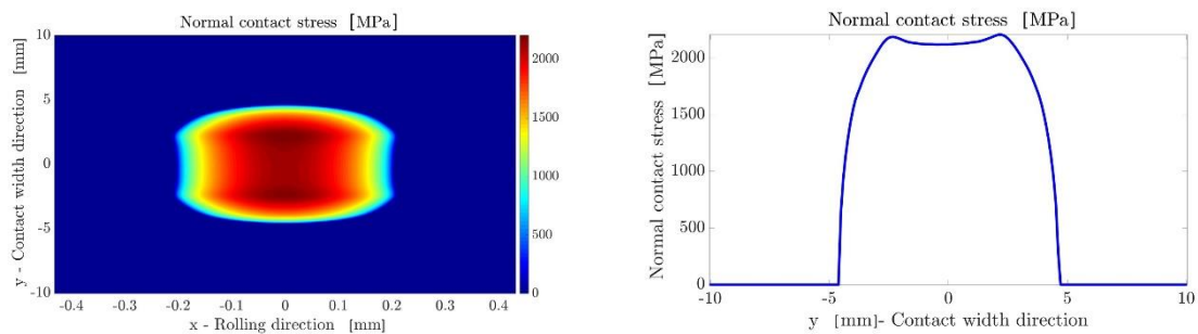
Figure 3: Exemplary presentation of the calculated normal contact stress distribution in the roller-washer contact of a cylindrical roller thrust bearing from type 81212 with 15 rolling elements under a constant axial load of 80 kN (parameter set 4 according to table 2)
