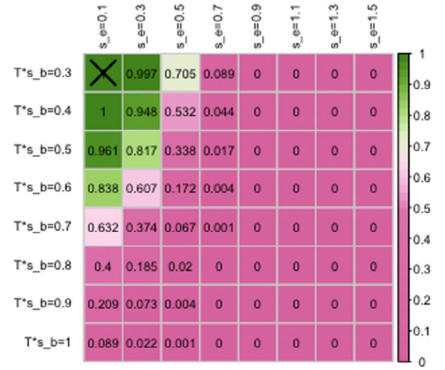
Large Degradation till T (bT=3), Assurance request q=0.99
