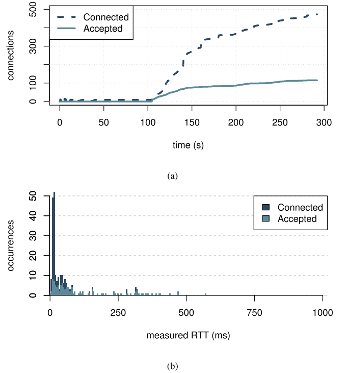
Fig. 2. The number of connected and accepted nodes with 99% Sybils (a) and a histogram of their latencies at the time of 300 s (b).
