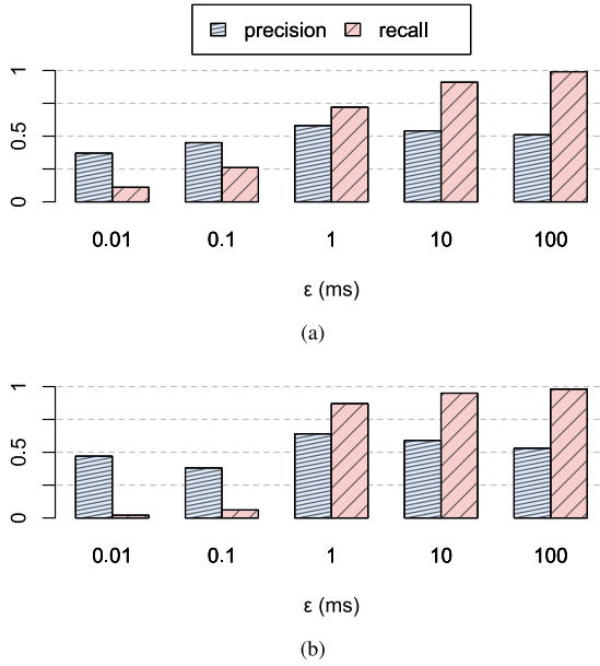
Fig. 7. The precision and recall for different values of \epsilon for the MSE classifier using the mean trendline (a) and the pivot trendline (b).
