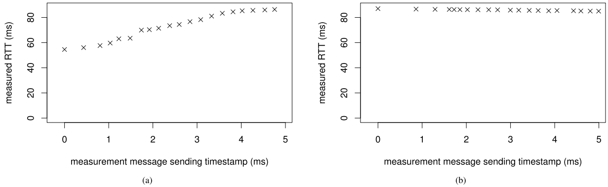
Fig. 4. The measured RTT per message sent in a single 20-message burst versus the message sending timestamp (starting from 0) for an honest node (a) and a Sybil (b).
