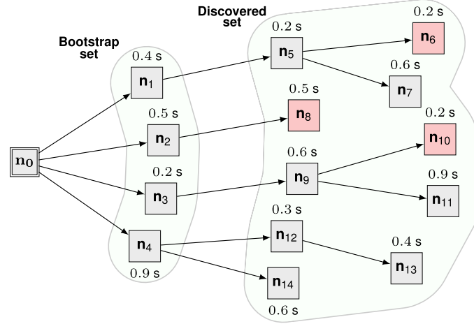
Fig. 5. Example of a peer discovery tree for a node n_0 with a maximum depth of 3 and \Delta = 0.1 s. Nodes with dark (red) shading violate the latency diversity. (For interpretation of the references to color in this figure legend, the reader is referred to the web version of this article.)
