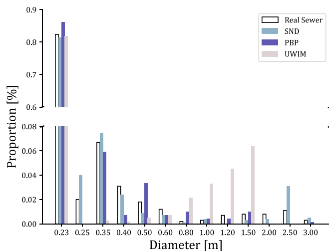
Fig. 4. Pipe diameter frequency distributions for the real and generated sewer networks using three design methodologies.
