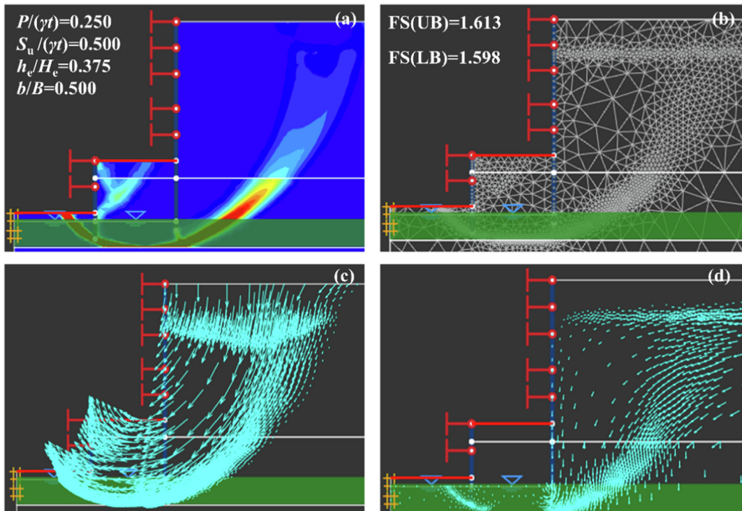
Fig. 6. Failure mode M2 of PIP braced excavation subjected to hydraulic uplift with P/(\gamma t) = 0.250 , S_u/(\gamma t) = 0.500 , h_e/H_e = 0.375 and b/B = 0.500 : (a) shear dissipation contours, (b) adaptive meshes, (c) incremental displacement vectors, and (d) groundwater flow vectors.
