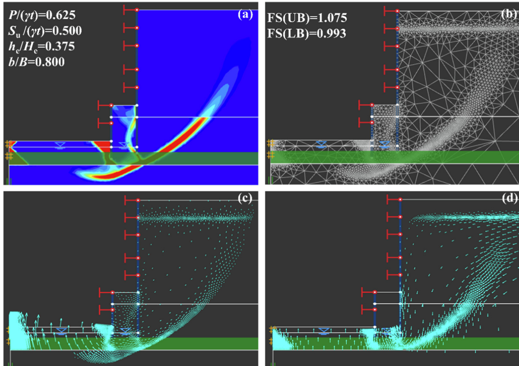
Fig. 8. Failure mode M4 of PIP braced excavation subjected to hydraulic uplift with P/(\gamma t) = 0.625 , S_u/(\gamma t) = 0.500 , h_e/H_e = 0.375 and b/B = 0.800 : (a) shear dissipation contours, (b) adaptive meshes, (c) incremental displacement vectors, and (d) groundwater flow vectors.
