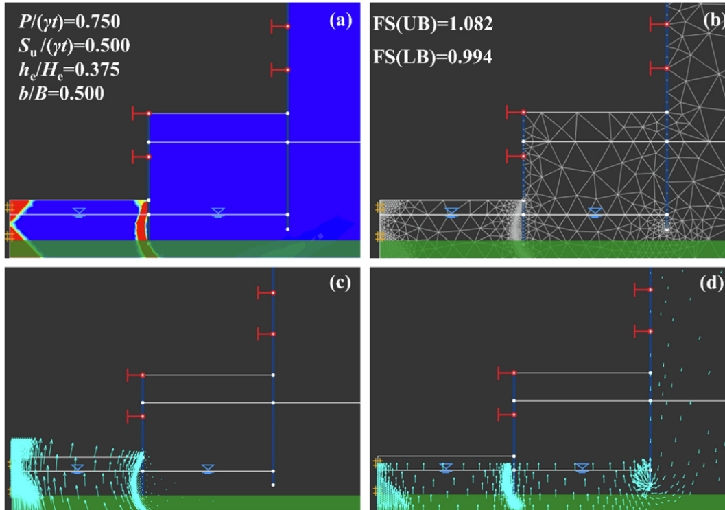
Fig. 9. Failure mode M5 of PIP braced excavation subjected to hydraulic uplift with P/(\gamma t) = 0.750 , S_u/(\gamma t) = 0.500 , h_e/H_e = 0.375 and b/B = 0.500 : (a) shear dissipation contours, (b) adaptive meshes, (c) incremental displacement vectors, and (d) groundwater flow vectors.
