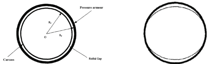
Fig.5 Progressive buckling process for a symmetrical collapse model [17]
