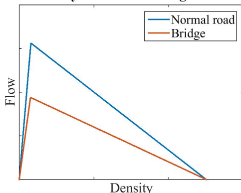
Helly fundamental diagrams
