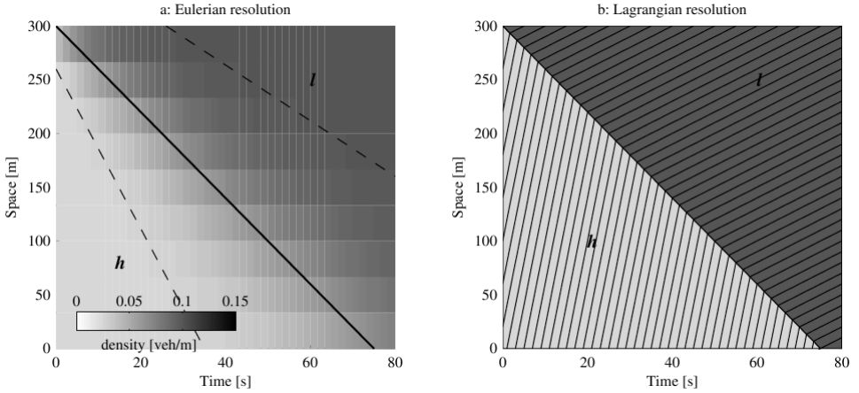
Figure 10.4: Simulation results of the backward propagation of a congestion tail, simulated in Lagrangian and Eulerian coordinates. Figure from Leclercq et al. (2007)
