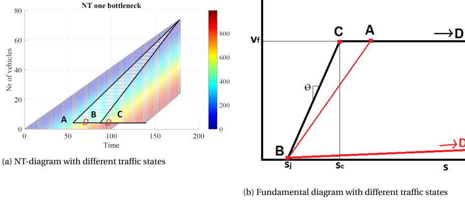
Figure 15.5: Shockwave Theory in the X-model, with different traffic states, A = inflow, B = jam, C = Capacity, D = empty road. Traffic state D is infinitely small.
