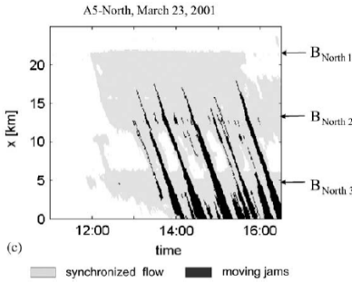
Figure 6.8: Observations of wide moving jams propagating through synchronised flow; figure from Kerner (2004)
