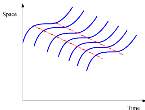
Figure 7.2: The average of the car-following behavior of drivers each with different parameters of the Newell model leads to a shock wave speed
