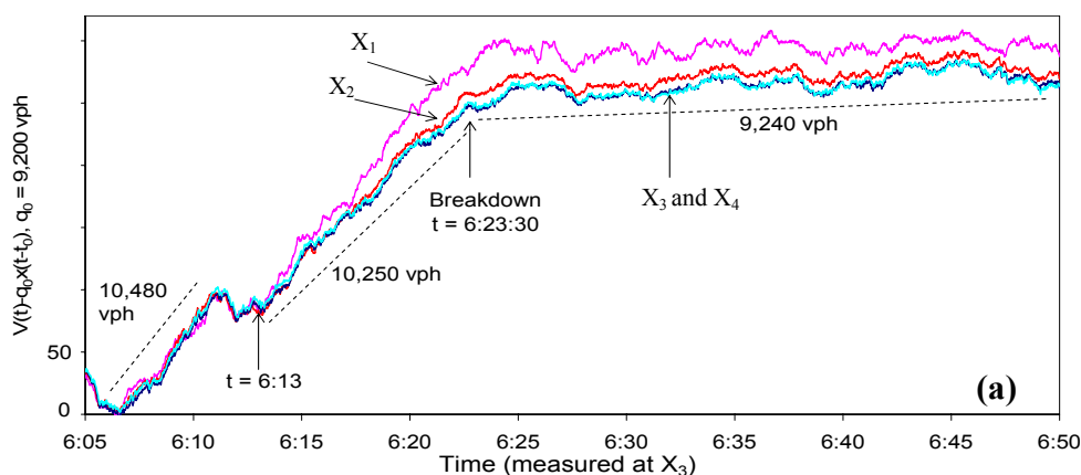
Figure 6.2: Example of an analysis with slanted cumulative curves, from Cassidy and Rudjanakanoknad (2005)
