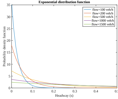
Figure 14.6: The probability density function for headways according to the exponential distribution for different flow values
