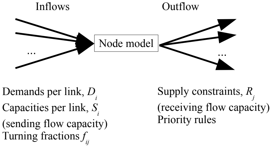
Figure 11.2: Node model structure
