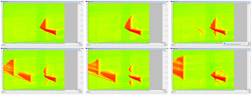
Figure 9.1: Examples of different random seeds in a simulation model. Colors indicate speed in a time-space plane (space is horizontal, time increases from bottom to top)
