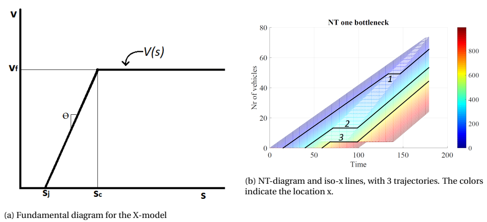
Figure 15.4: Representation of traffic in the X-model
