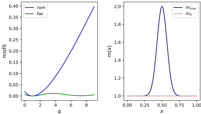
Fig. 1 Comparison between the ROM based FWI and the conventional FWI when we use 10 wavenumbers with k_{\min} = 18 and k_{\max} = 24 . On the right we show m_0 and m_{\text{true}}
