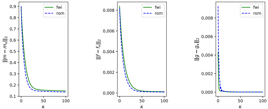
Fig. 8 From left to right. On the left, comparison of the misfit \|m - m_K\|_2 when m_K is recovered doing \kappa -steps of the fixed point iterations either of the conventional or the ROM based FWI method. We compare similarly the misfits of the reflection and the transmission data yielded by the respective m_K . We used the same step \omega in both fixed point iterations
