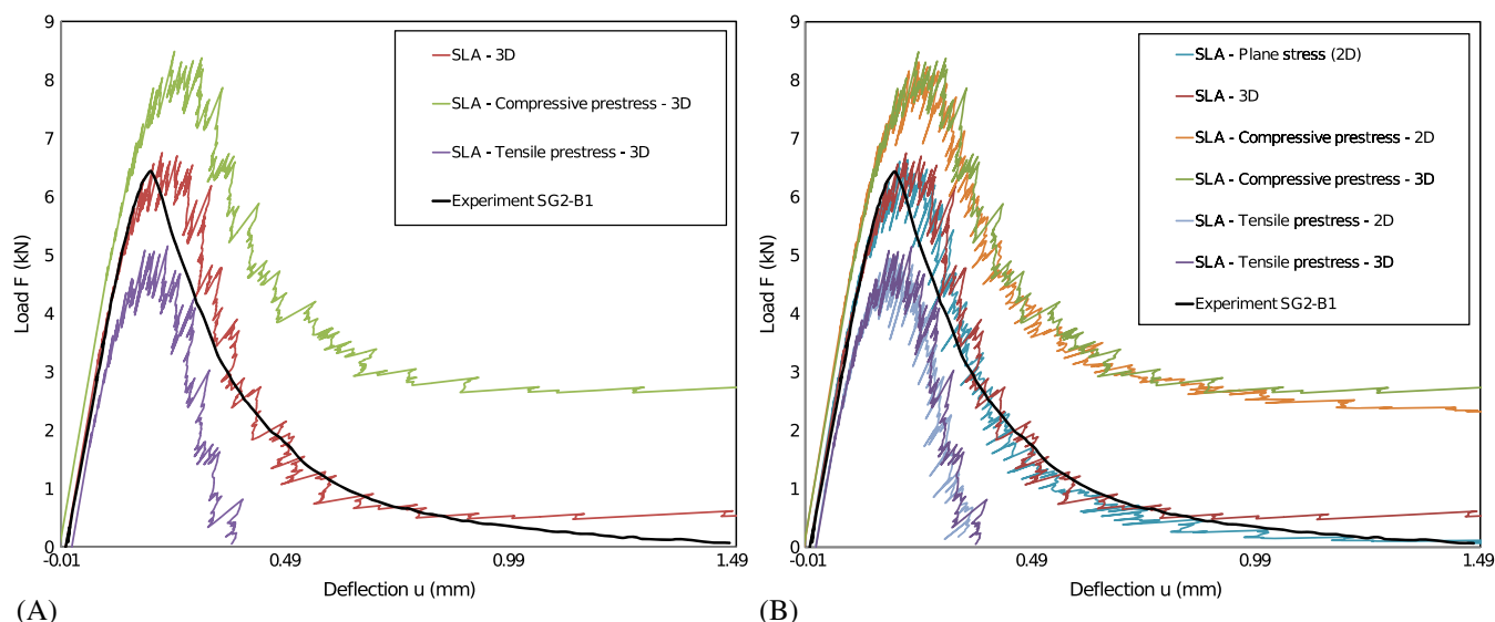
FIGURE 5 (A) Force displacement curves for the three-point bending cases using the three-dimensional (3D) model with and without axial loads and (B) its comparison against two-dimensional (2D) plane stress state simulations. SLA, sequentially linear analysis
