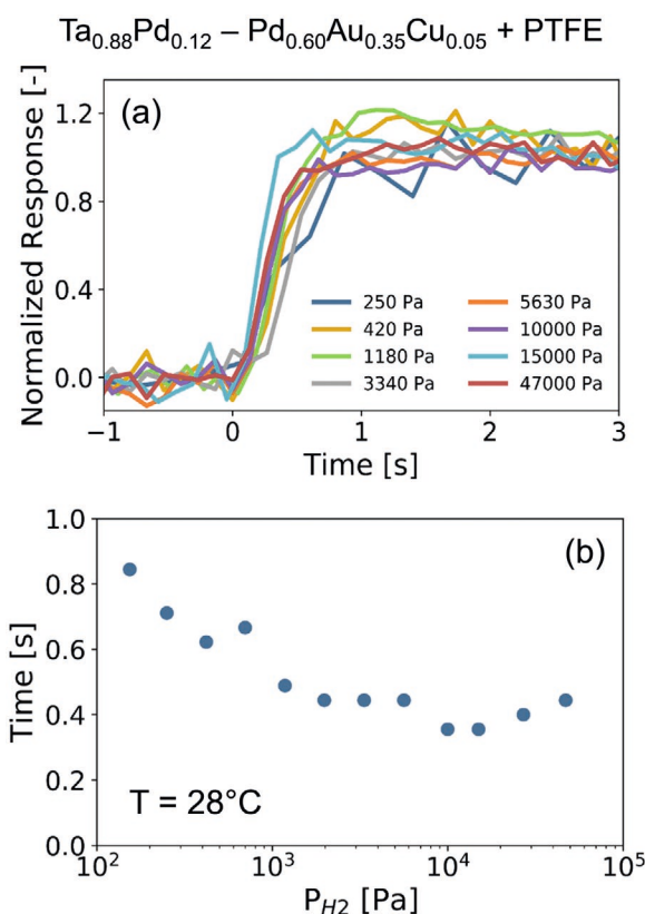
Figure 5. Absorption kinetics of a 40 nm \text{Ta}_{0.88}\text{Pd}_{0.12} thin film with a 4 nm Ti adhesion layer capped with a 10 nm \text{Pd}_{0.60}\text{Au}_{0.35}\text{Cu}_{0.05} layer that is covered with a 30 nm PTFE layer (" \text{Ta}_{0.88}\text{Pd}_{0.12} - \text{Pd}_{0.60}\text{Au}_{0.35}\text{Cu}_{0.05} + \text{PTFE} ") at T = 28^\circ\text{C} . a) Normalized responses of the thin film to a series of pressure steps between P_{\text{H}_2} = 0.5 \times 10^2 Pa and the partial hydrogen pressure indicated. b) Hydrogen pressure dependence of the response time of the thin film. The response time is defined as the time to reach 90% of the total signal.
