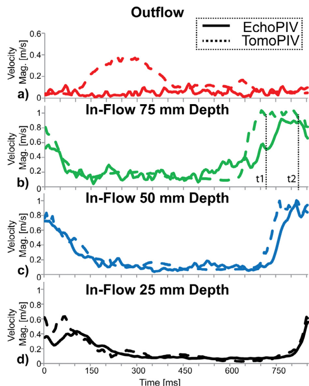
Fig. 8. Velocity magnitude comparison through a 4 mm diameter sphere in the center of the jet at different depths (the same depths as indicated in Fig. 7a). Solid/dashed lines represent the average velocity magnitude for echo-PIV and tomo-PIV. Note that echo-PIV underestimates velocities more at farther distances from the probe. Time points t1 and t2 shown again for clarity; see Figure 9 for velocity profiles these times.
