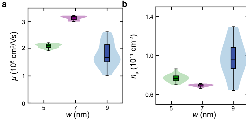
Figure 2.2: Electrical transport characteristics. a, b Distributions of mobility \mu measured at n = 6 \times 10^{11} \text{ cm}^{-2} and percolation density n_p for heterostructures featuring quantum wells of different thickness w : 9.0(5) nm (blue, heterostructure A, 16 Hall bars measured and reported in ref. [3]), 6.9(5) nm (purple, heterostructure B, 10 Hall bars), and 5.3(5) nm (green, heterostructure C, 22 Hall bars measured and reported in ref. [3]). Violin plots, quartile box plots, and mode (horizontal line) are shown.
