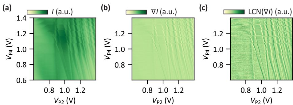
Figure 6.20: Processing of the data underlying Fig. 6.7.b. (a) Sum of the sensor response I of the charge stability diagrams shown in Fig. 6.19. (b) Gradient \nabla I of the data shown in (a). (c) Final signal LCN(\nabla I) after applying a local contrast normalization to the map shown in (b).
