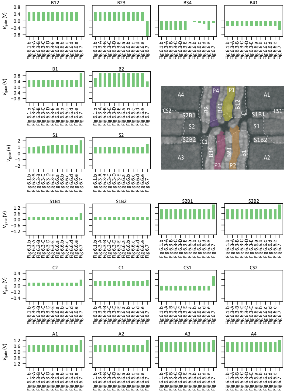
Figure 6.21: Gate voltage evolution during the presented experiments. Each panel shows the gate voltage evolution of a single gate during the experiments presented in Fig. 6.1-6.7 as given on the x-axis. Note that V_{S2C} = 0 V during all experiments. The inset shows an SEM image of a device nominally identical to the one under study. Confinement gates are outlined by a white dashed line. Labels indicate the gate electrode naming convention utilized throughout the chapter and in the panels of this figure.
