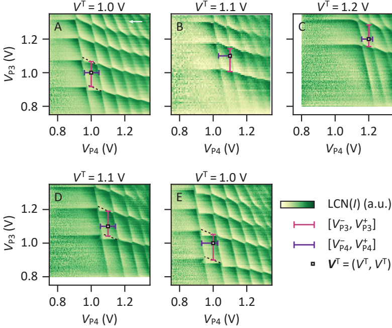
Figure 6.3: Evolution of charge stability regions under voltage stressing. Charge stability diagrams recorded after the application of the respective stress voltage sequences. The white square markers show the target voltages \mathbf{V}^T = (V^T, V^T) . Plunger gate voltage ranges [V_{P_i}^-, V_{P_i}^+] that keep the system in the (1,1) charge state are indicated by vertical and horizontal bars. Dashed lines indicate transitions of the charge ground state which cannot be observed directly due to a slow dot-reservoir tunneling time of Q3 (charge latching, see section 6.4). The white arrow marks the sweep direction which is identical for all panels. Unprocessed data shown in section 6.11.
