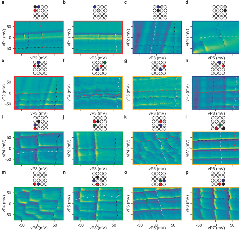
Figure 4.25: Tune-up of the crossbar array in the few-holes regime. a-p , Charge stability diagrams (raw sensor signal after subtraction of a background) showcasing the 16 quantum dot system in the few-hole regime. These measurements are taken in the first tune-up of the crossbar array. In each map, the first visible transition lines from the right or the top are labelled and assigned to the relative quantum dot by dashed lines with colours defined in the schematic at the top. The identification is performed via the results of Fig. 4.12-4.16. The colour of the panel frame identifies the sensor used: NW in red, NE in blue, SW in green, and SE in ochre.
