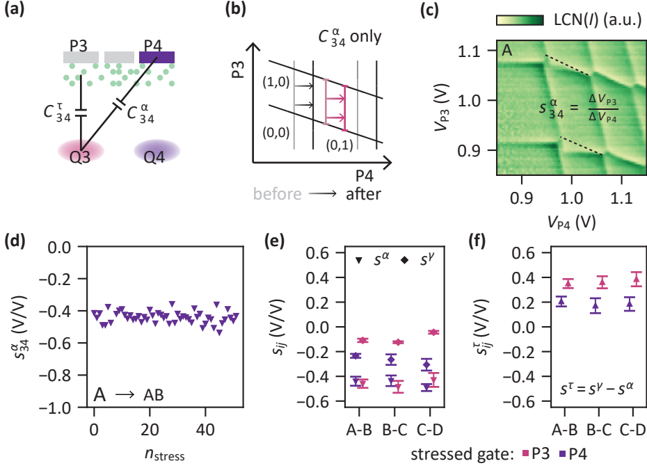
Figure 6.9: Stress tuning crosstalk and cross-capacitance effects. (a) Illustration of a device cross-section portraying the capacitive effect of the plunger gate voltage V_{P4} on the potential of quantum dot Q3 ( C_{34}^{\alpha} ) and the crosstalk effect of applying stress voltages to plunger gate P4 on the potential of quantum dot Q3 ( C_{34}^{\tau} ). (b) Schematic charge stability diagram illustrating how the charge transition voltages of quantum dot Q3 shift when changing the voltage on plunger gate P4. Grey lines indicate the charge transition lines before and black lines after changing the potential of Q4 through applying stress voltages. For illustration purposes, the interdot coupling between Q3 and Q4 and the capacitive coupling of P3 onto Q4 are neglected. (c) Example charge stability diagram taken at point A in Fig. 6.8.a. The slope s_{34}^{\alpha} of the transition lines of Q3 (black dashed lines) are determined as a measure for the relative capacitive effect of plunger gate P4 onto the potential of quantum dot Q3. To ensure robustness against distortions from charge latching effects, the Q3 charge transition lines are defined as the lines connecting the respective triple charge degeneracy points. (d) All extracted s_{34}^{\alpha} during the tuning from point A to AB in Fig. 6.8.a. (e) Crosstalk s_{ij}^{\gamma} caused by stressing plunger gate P_i (diamonds) and cross-capacitance effect s_{ij}^{\alpha} of plunger gate voltage V_{P_j} (downward pointing triangles) onto the potential of quantum dot Q_i along the trajectory in Fig. 6.8.a. Between C and CD and CD and D only the last ten points are fitted to extract s_{ij}^{\gamma} . Due to a limited number of data points, no values are shown for the tuning between D and E. (f) Stress voltage induced crosstalk effect s_{ij}^{\tau} of plunger gate P_j onto the potential of quantum dot Q_i corrected for the capacitive coupling of plunger gate P_j onto the potential of quantum dot Q_i .
