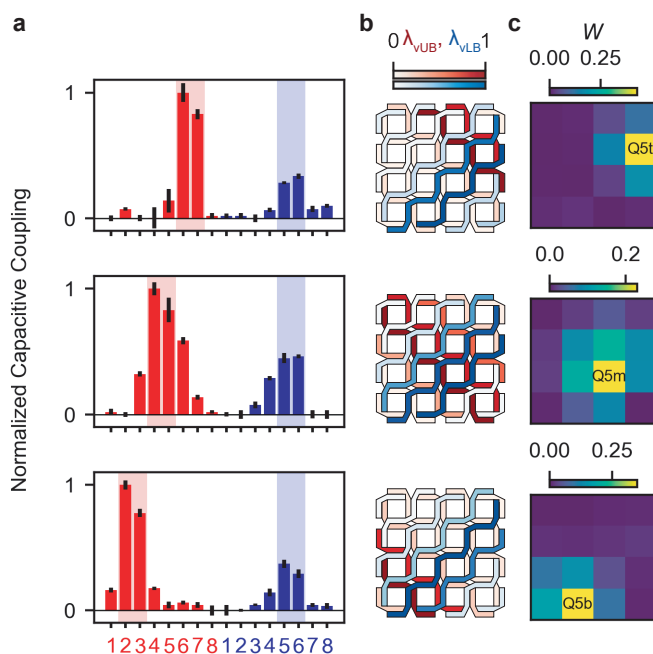
Figure 4.14: Quantum dot identification of the Q5 quantum dots Same as in Fig. 4.12 but applied to the Q5 quantum dots. The three different rows of panels a , b , c enable to label the Q5 quantum dots.
