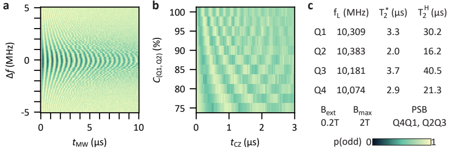
Figure 7.2: Spin manipulation in the 2 \times 2 array. a) EDSR-driven Rabi oscillations of the spin in quantum dot Q1. A typical Chevron pattern is obtained as a function of pulse duration t_{MW} and the drive frequency detuning \Delta f = f_L - f_{MW} where f_L is the qubit Lamor frequency and f_{MW} is the applied microwave signal frequency. The microwave pulse is applied to the lower screening gate labeled S23 in chapter 3. Initialization and readout are based on PSB parity readout and post-selection [7] on readout pair (Q4, Q1). b) Decoupled CZ gate [11] applied to Q1 and Q2 and as a function of interaction time t_{CZ} and coupling strength C_{(Q1,Q2)} = (vB12 - vB12_{min}) / (vB12_{max} - vB12_{min}) with vB12_{min} and vB12_{max} barrier voltages corresponding to an exchange interaction of f_j \lesssim 20 kHz and f_j \gtrsim 1 MHz, respectively. The spins in Q1 and Q2 are initialized followed by a \pi/2 rotation around the x-axis of Q1 (noted as X_1(\pi/2) ). Then two adiabatic controlled phase gates of duration t_{CZ} interleaved by refocusing X_1(\pi) and X_2(\pi) pulses are applied. Finally, a X_1(\pi/2) and a X_2(\pi) pulse are followed by PSB readout on quantum dot pair (Q4, Q1). c) Table summarizing all four Lamor frequencies f_L , coherence times T_2^* and Hahn echo times T_2^H as well as providing the applied B-field B_{ext} , the maximum applied B-field to magnetize the micromagnet B_{max} and the quantum dot pairs used for PSB readout. The quantum dots and gate electrodes are named as in chapter 3. For instance, quantum dot Q1 is located at the upper right of the array. The device is tuned to the (1,1,1,1) charge state with one electron per quantum dot.
