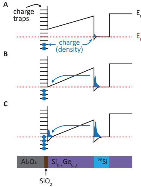
Figure 2.7: Charge tunneling from the quantum well to the dielectric interface. A cross-section through a Si/SiGe devices is shown (bottom). The shape of the conduction band energy ( E_C ) and Fermi level ( E_F ) in this heterostructure for three regimes (A-C) of gate voltages is drawn above. Interface traps are depicted by horizontal lines and their occupation is indicated by blue circles. The charge density across the material stack is depicted in blue. For low to moderate gate voltages (A) the conduction band is pulled below the Fermi energy and electrons accumulate in the Si quantum well. For increased gate voltages (B) electrons can tunnel from the quantum well through the SiGe buffer as indicated by the blue arrow and occupy interface charge traps. Under the application of even higher gate voltages (C) electrons accumulate directly at the silicon oxide interface. Figure inspired by refs [90], [108], [109].
