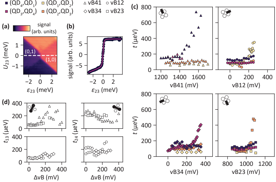
Figure 3.4: a) Exemplary charge stability diagram around the (1,0) to (0,1) transition for QD 2 and QD 3 as a function of the interdot detuning \epsilon_{23} and U_{23}/\alpha U_{23} = vP_2 + vP_3 . The dashed line indicates the detuning axis used to measure polarisation lines. b) Example of a measured (dots) and fitted (solid line) polarisation line for QD 2 and QD 3 . c) Dependence of the tunnel couplings extracted from polarization lines between neighbouring quantum dots on each of the four virtual barrier gate voltages. The plots are ordered to follow the physical position of the barrier gate e.g. barrier vB 41 situated in the top left corner of the quantum dot array is depicted in the top left plot. The legend for symbols and colors is shown above panels a) and b). We note that the dc voltages of barriers vB 12 (vB 23 ) and vB 34 (vB 41 ) are of comparable values, which is consistent with the symmetries of the gate pattern. Between scans we adjusted gate voltages of uninvolved gates to retain a high visibility. These adjustments were done in such a way that all uninvolved barrier gates remained in the small (residual) tunnel coupling regime. On several occasions, insufficient contrast between the (1,0) and (0,1) charge states limited the data we were able to reliably fit. These data points are thus not available. d) Diagonal tunnel coupling and anti-diagonal tunnel coupling as a function of all four virtual barrier gate voltages. The panels were split into two parts for both the diagonal and anti-diagonal coupling to keep the data points visible. The physical gate voltages used at \Delta vB = 0 mV varies between data sets, as the voltages were slightly adjusted. As in c) uninvolved barrier gates remained in the residual tunnel coupling regime. Note also that in c) and d) the charge states vary between scans, depending on which dots each polarization line connects.
