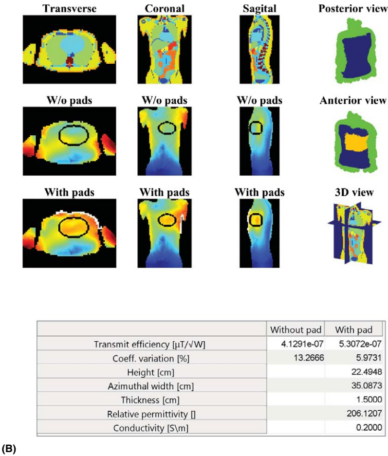
FIGURE 4 Design procedure for imaging the heart at 3T. A, The result is shown for a parameter sweep over a predefined set of target fields, after which a desired design can be selected based on the efficiency-homogeneity plot. For the selected design (here, number 5), a single optimization is performed to obtain the results as shown in (B) for later reference. Design number 7 is not chosen here, as the dimensions of the dielectric pad are not practical. The lookup table for the individual simulations can be found in Supporting Information Table S1
