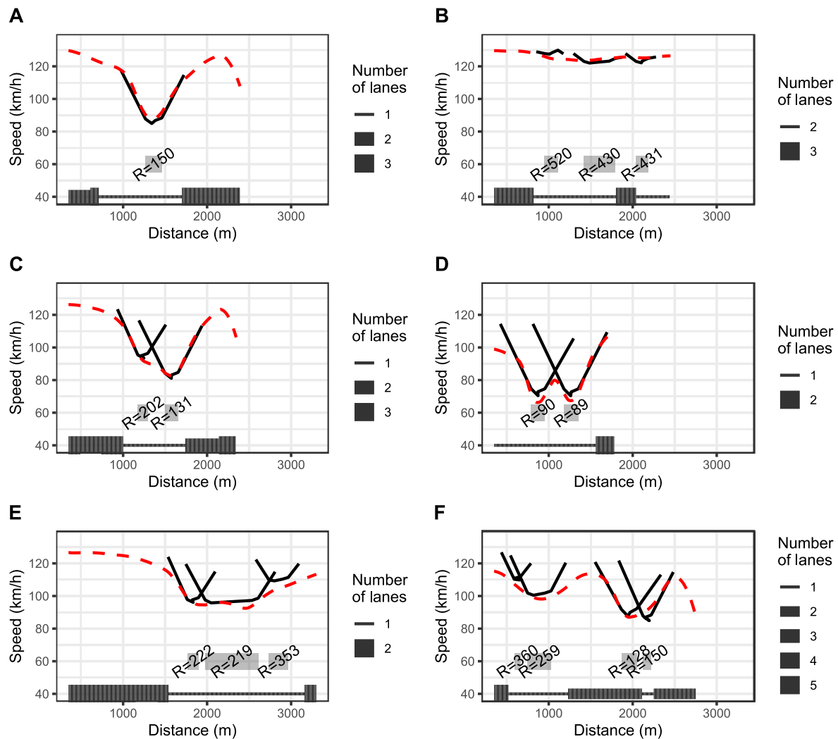
Figure 4-8 Observed and predicted speed profiles; red dashed line is the observed 85 th percentile speed, the black lines are the predicted speed profiles per curve. Curve radii in a grey box representing the position of the curve. Below that a line indicating the number of lanes present along the profile.
