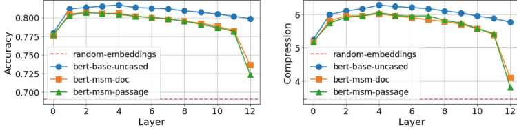
Fig. 4. Probing results over the layers for the NER task.
