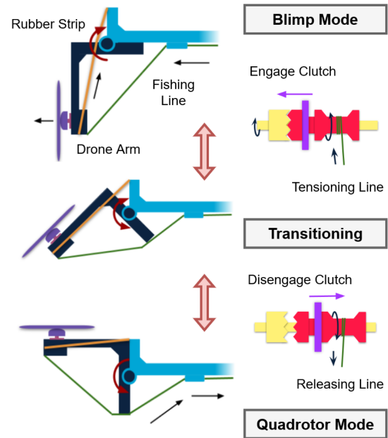
Fig. 3. Janus morphing mechanism transitions the blimp into a regular quadrotor via a reel and clutch system.
