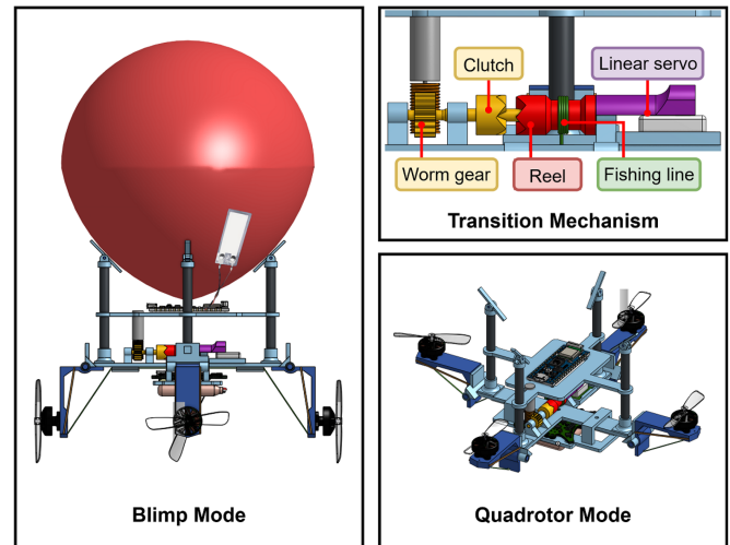
Fig. 2. Janus can morph between two modes: a blimp and a quadrotor, using a specially designed transition mechanism.
