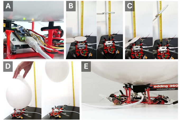
Fig. 8. False positive scenarios considered with a proximity sensor: (a) IR LED, (b) horizontal mirror, (c) 45° angled mirror, (d) different coloured balloons and (e) swiping different reflective objects like marker cap.
