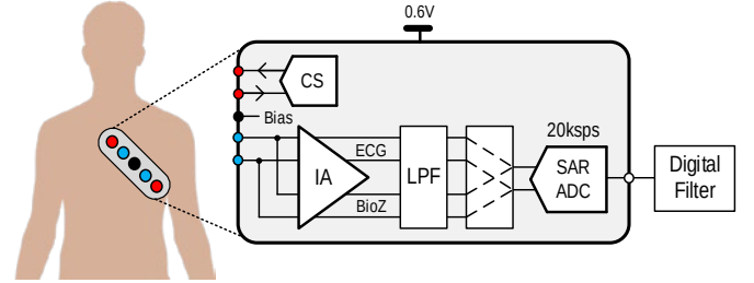
Fig. 1. IC block diagram and simultaneous ECG and BioZ measurement with one single amplifier
