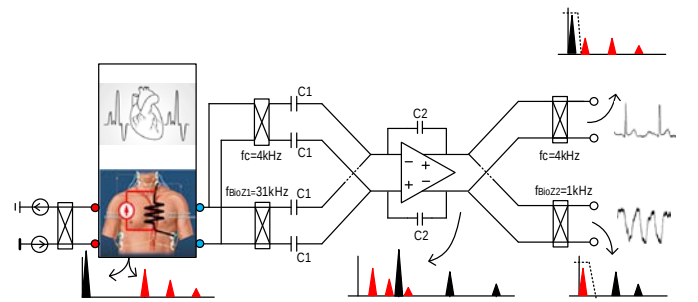
Fig. 2. Simultaneous ECG and BioZ measurement with one single amplifier
