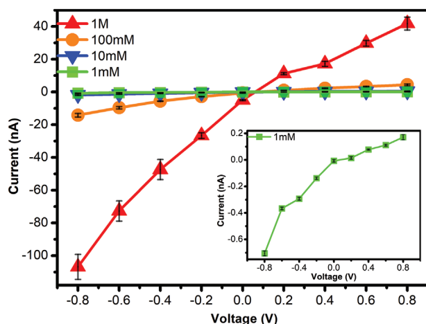
Figure 3. Typical current–voltage curves of an ionic FET based on silicon nanopore with a feature size of 6 nm in KCl electrolyte concentration from 0.001 to 1 M (pH 7.2) and applied bias voltage from −0.8 to 0.8 V.
