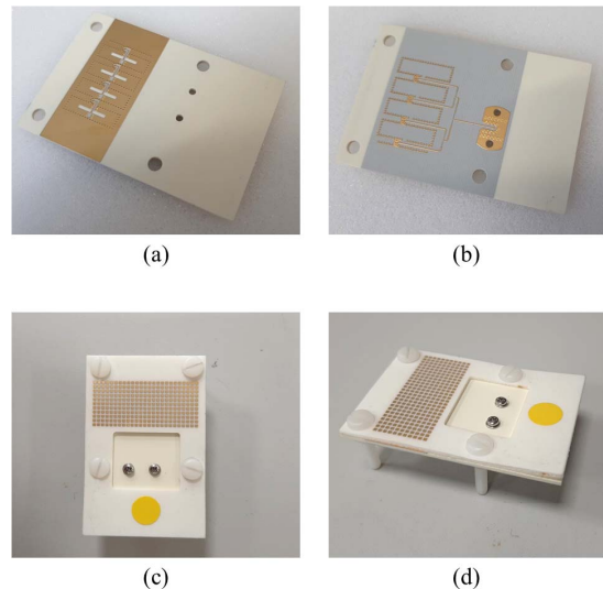
Fig. 13. Photographs of fabricated demonstrator boards. (a) Top view of array without ADL superstrate. (b) Bottom view of broadside board. (c) Top view of assembled PCBs. (d) Overview of assembled PCBs.
