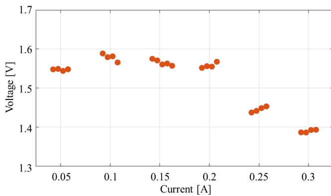
Fig. 6: The MVTP voltages at each applied current. The data points per applied current level are in chronological order.
