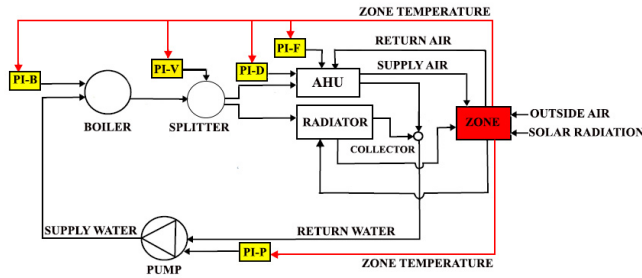
Fig. 1: HVAC system and control architecture
