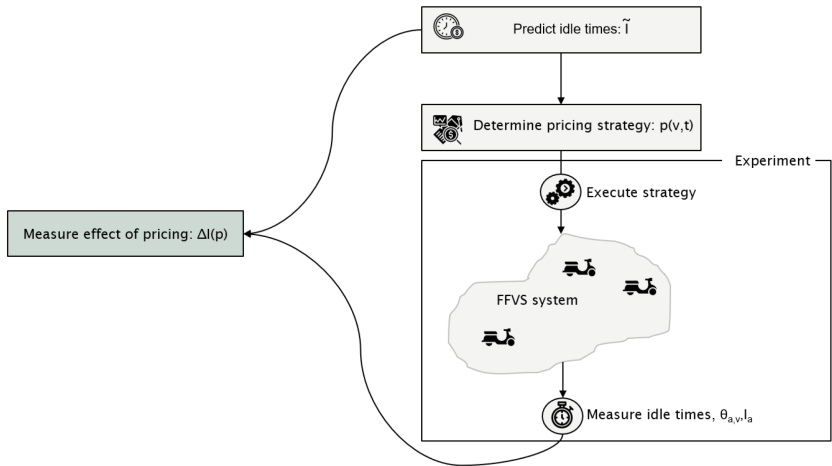
Fig. 3. The expected idle times are used to determine a pricing strategy. The execution of this strategy will then result in idle times which can be compared with the expected idle times. The comparison of the resulting values and expected values will show the effectiveness of a strategy.
