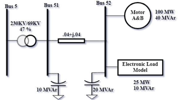
Fig. 3: Composite load model as specified in
