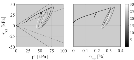
Figure 7. Soil shear stress-strain response and effective stress path 4 m right of the monopile and 3.6 m below the mudline (scenario C).
