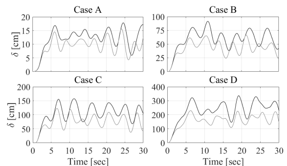
Figure 9. Displacement time histories at the OWT hub.
