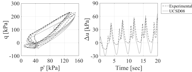
Figure 6. UCSD08 simulation a cyclic two-way triaxial test (initial effective stresses \sigma'_{ov}=187 kPa and \sigma'_{oh}=90 kPa).
