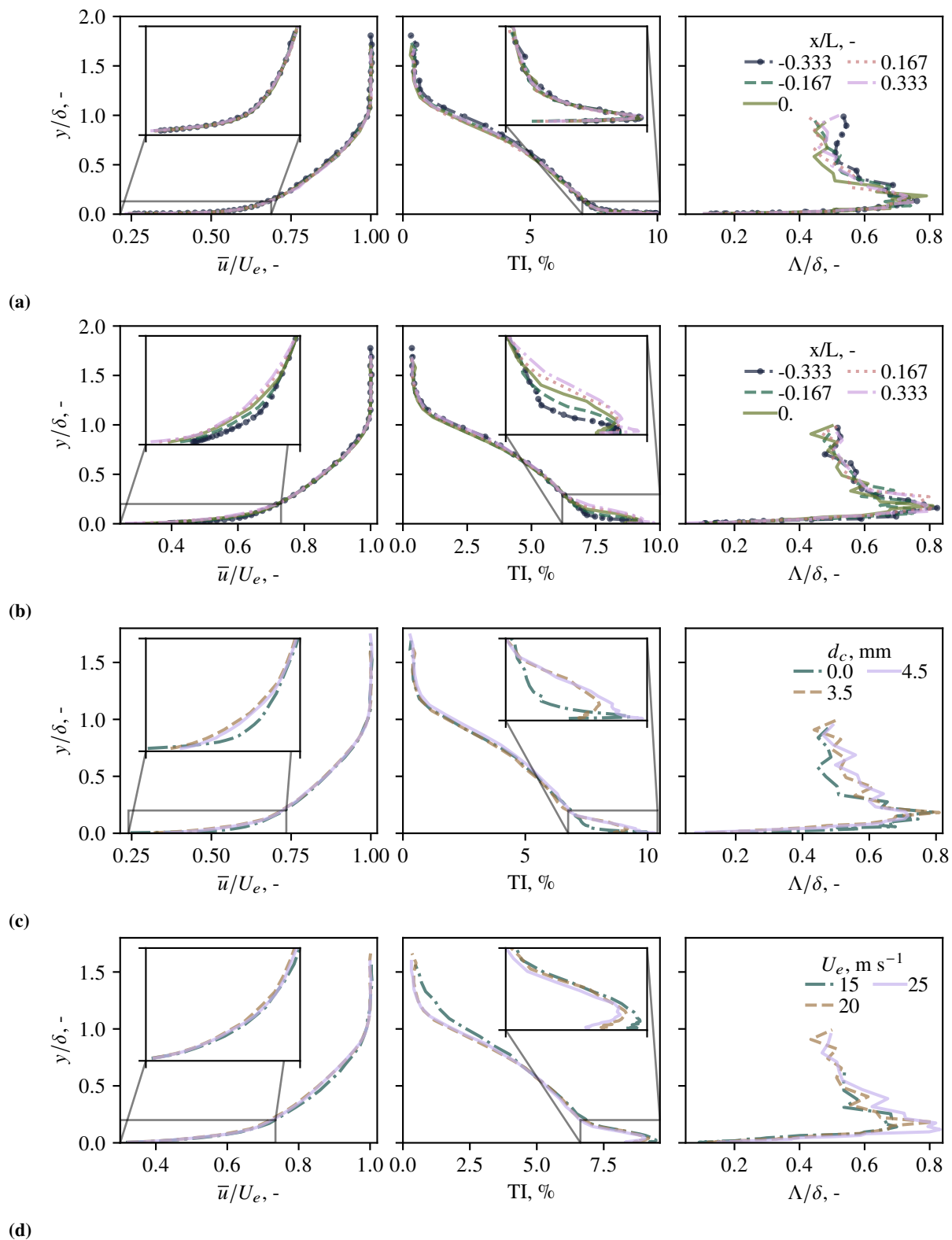
Fig. 9 HWA measurements. When not otherwise stated, the conditions are: d_c = 3.5 mm, U_e = 20 \text{ m s}^{-1} , and x/L = 0 . (a) Solid-walled case d_c = 0 mm; (b) Effect of x/L ; (c) Effect of d_c ; (d) Effect of U_e .
