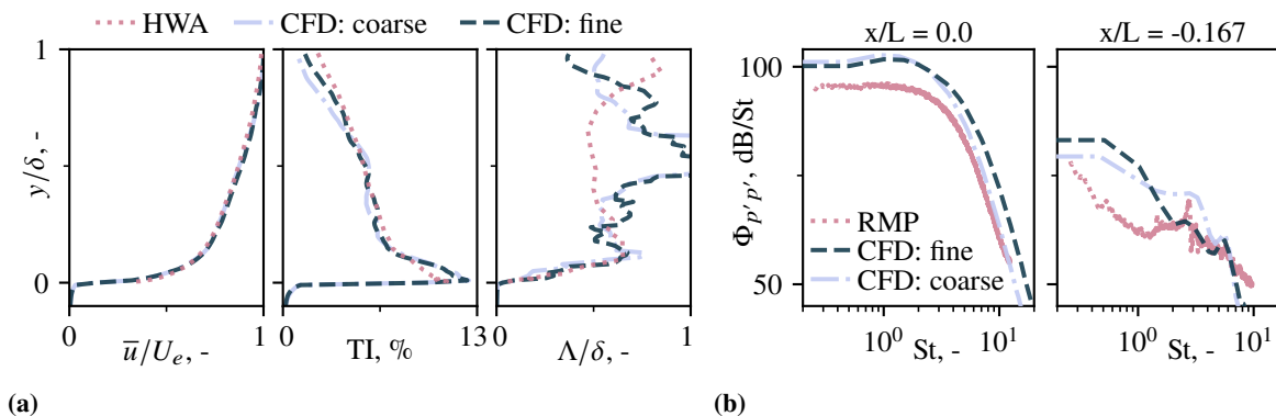
Fig. 5 Comparison between wind-tunnel measurements (HWA and WPS) and simulation data with the standard, i.e., fine , and the coarse mesh. The conditions are d_c = 4.5 mm and U_e = 15 m s -1 . (a) Boundary-layer profiles for x/L = 0 ; (b) WPS on the upper ( x/L = 0 ) and lower surface ( x/L = -0.167 ) of the porous wall-insert.
