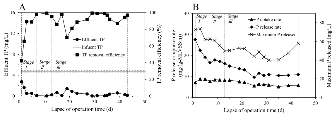
Fig. 6. Changes in effluent TP concentration and TP removal efficiency (A), and P release and uptake rates during the three operational stages (B).
