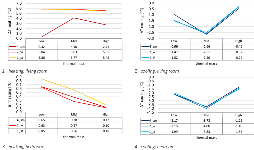
FIGURE 5.3 Heat-up-speed and Cool-down-speed 95% percentiles living room and bedroom for adaptive heating (Table 5.6); \Delta T = temperature difference to be made by heating or cooling from one time-step to the next at change of setpoint temperature, maximum in 95% of the time
