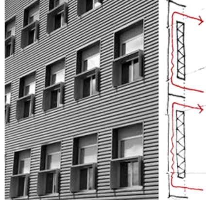
2 Application of collector wall (in opaque façade parts) RNEL (DeFreitas, 2010)
