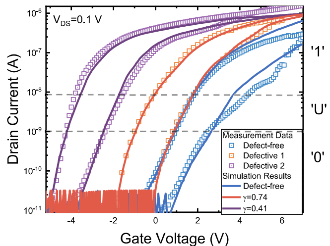
Fig. 1: Measurement and fitting of defective I_d - V_g under the same conditions. The parameter \gamma is introduced in Equations 5-6 and denotes a specific, time-independent defect strength for each device.
